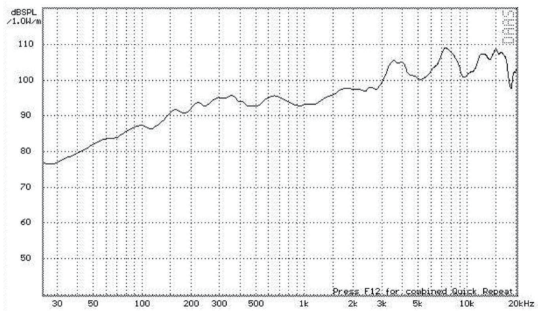
MEASUREMENTS WITHOUT GRILLE
