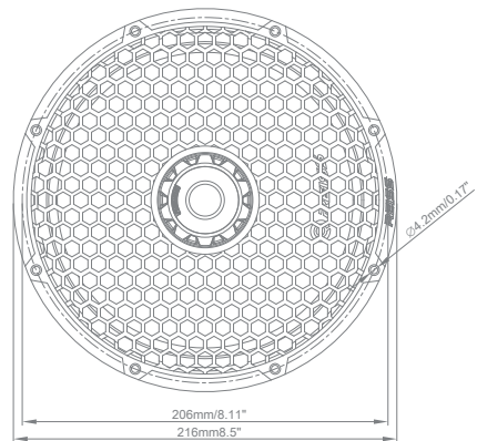
MEASUREMENTS WITH GRILLE
