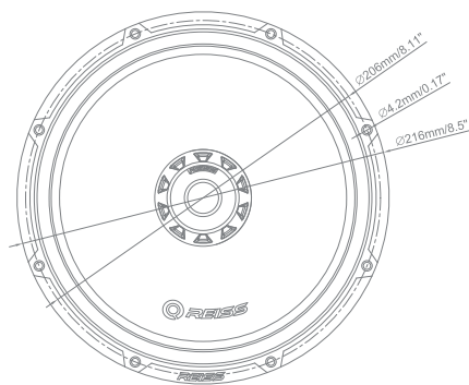
MEASUREMENTS WITHOUT GRILLE
